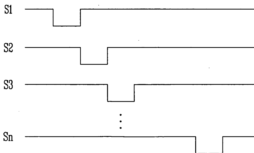
FIG. 2 (PRIOR ART)
